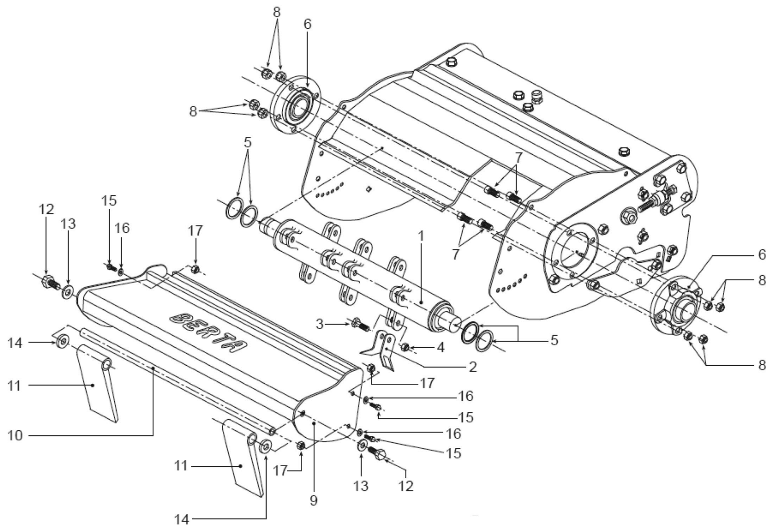
Berta Flail Attachment - Rotor
