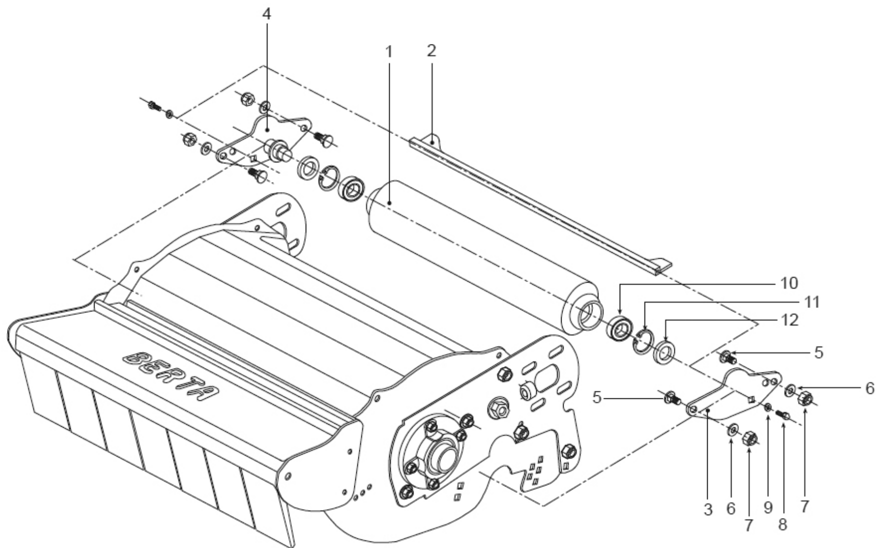
Berta Flail Attachment - Roller
