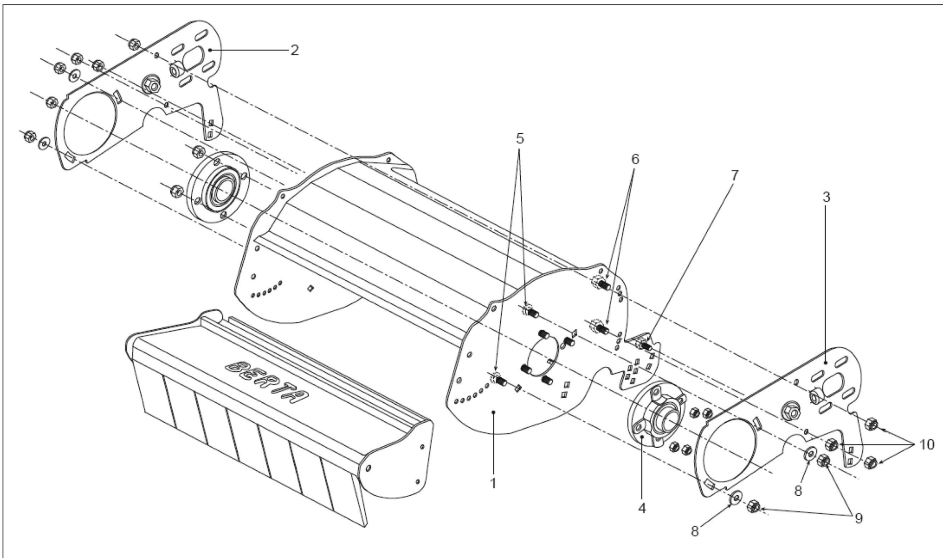
Berta Flail Attachment - Main Body
