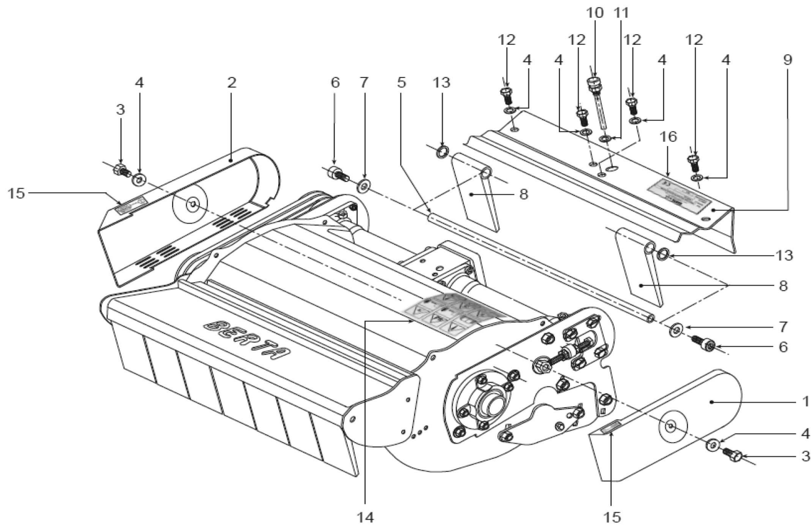
Berta Flail Attachment - Cover
