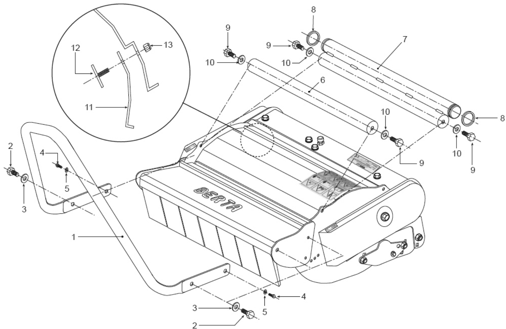
Berta Flail Attachment - Frame
