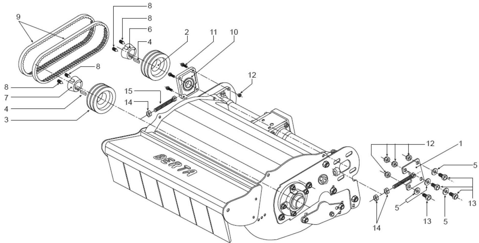
Berta Flail Attachment - Pulley
